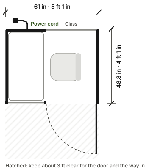
PLAN, FRONT AT THE BOTTOM FURNITURE INDICATIVE
